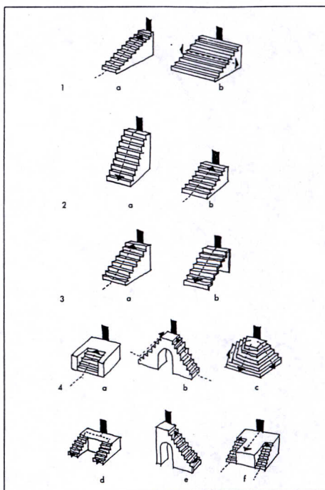
Thomas Thiis-Evensen's Archetypes of Architecture (see p. 6) is a major contribution to an experiential graphics. In this drawing, he illustrates the four qualities that contribute to how one experiences a particular stair: breadth—narrow (1a) or wide (1b); slope—steep (2a) or gentle (2b); attached (3a) or free-standing (3b); form—plateau (4a), frontal (4b), fan (4c), divided (4d), side (4e), or overlapping (4f).
